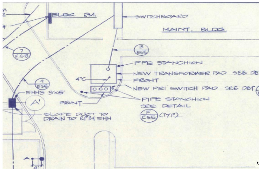
Figure 1: Site Plan.
