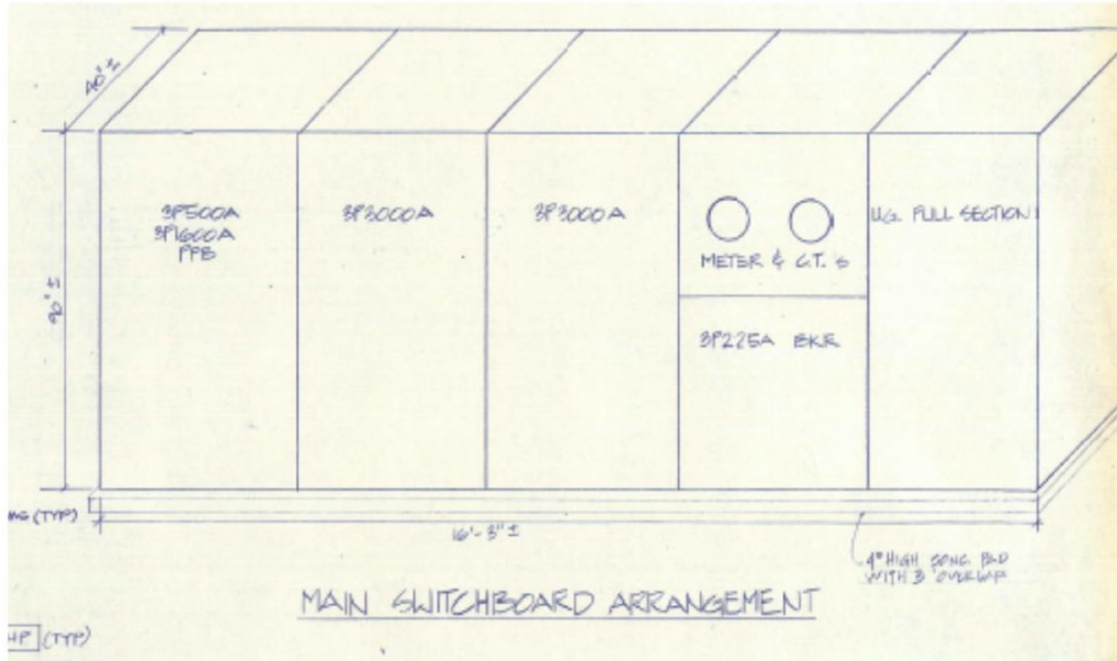
Figure 2: Existing Main Switchboard Arrangement
